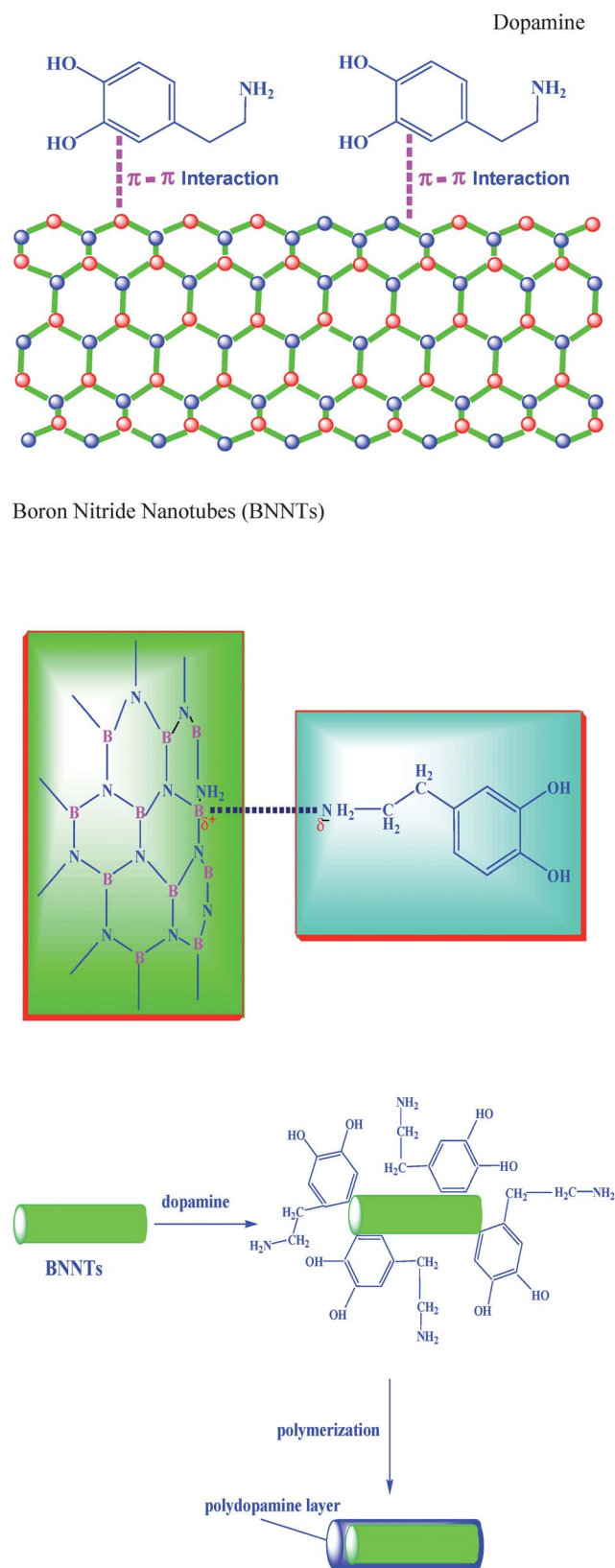
Scheme 1 Schematic illustration of dopamine functionalization of BNNTs.
