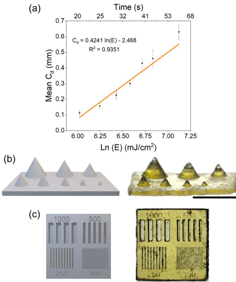
Figure 3. Jacobs working curves of the PBG resin and printed objects used to investigate print fidelity. (a) Working curve obtained from the Asiga printer. (b) Cones of varying radii (from far-left corner radii were 1.5, 1.25, 1.0, 0.75, 0.625, 0.5, 0.375, and 0.25 mm) on a rectangular plate, (c) Optimization chip with channels (areas where resin was uncured) and features (lines between channels that were cured) that were 1000, 500, 250 and 100 \mu\text{m} in width and 0.6 mm in depth. Scale bars are all 5 mm scale.
