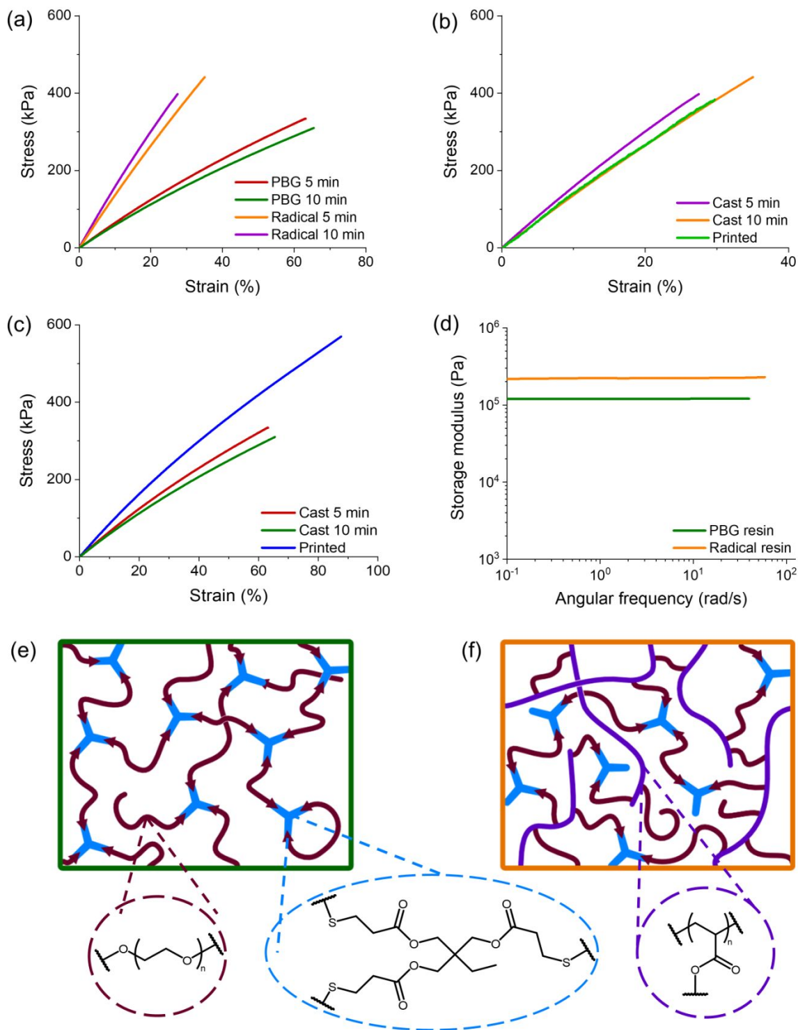
Figure 4. Mechanical properties comparing radical and PBG resins. (a) tensile experiments comparing cast dogbones of radical-mediated resin to base-catalyzed resin. (b) Comparing printed vs cast dogbones of radical-mediated resin. (c) Comparing printed vs cast dogbones of base-catalyzed resin. (d) Frequency sweeps comparing the gels made with radical and PBG resins. Schematic representations of (e) the base-catalyzed network and (f) the radical-mediated network.
