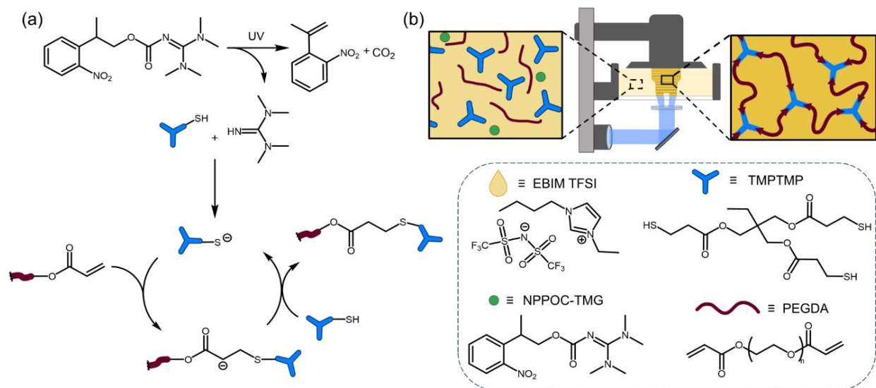
Figure 1. Base-catalyzed thiol-Michael DLP printing (a) reaction mechanism for photolysis of PBG and thiol-Michael reaction, (b) cartoon of DLP printer and chemical structures of resin components.
