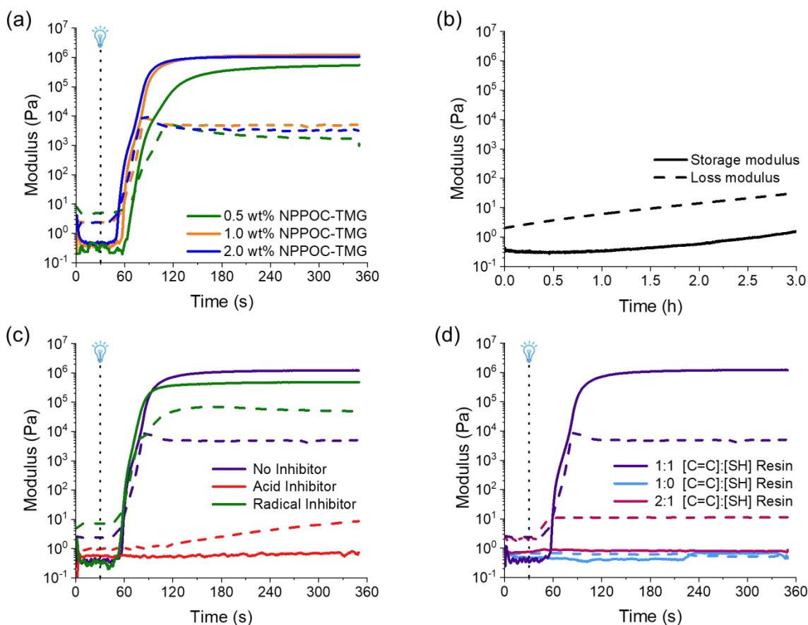
Figure 2. Rheology of thiol-Michael resins; dashed lines are G'' and solid lines are G' . Rheological conditions for photorheology: 1 Hz, 1% strain, Light on at 30 s. (a) UV curing experiment showing the effect of NPPOC-TMG concentration. (b) Dark stability of the resin (5 Pa strain amplitude, no light, 3 h). (c) UV curing of resins with radical inhibitor or organic acid. (d) UV curing comparing resins without trithiol monomer and substoichiometric thiol content.
