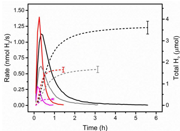
Fig. 3 Rates (solid lines) and amounts of H 2 (dashed lines) for homo- and heterogeneous photocatalytic reactions in 1 M ascorbate buffer (pH 4) with 0.1 M NaOTf. Black: 20 μM PS 5 and 1 μM WRC 3 immobilized on f-SiO 2 -C 18 with 300 μM 7 . Red: 20 μM [Ru(bpy) 3 ]Cl 2 and 1 μM 1 . Grey: 10 μM PS 5 and 0.5 μM WRC 3 immobilized on f-SiO 2 -C 18 with 150 μM 7 . Magenta: 10 μM [Ru(bpy) 3 ]Cl 2 and 0.5 μM 1 . Detailed values are shown in Table 1.
