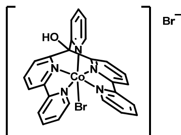
Scheme 1 Structure of water reducing catalyst [\text{Co}^{\text{II}}\text{Br}(\text{appy})]\text{Br} 1 . 52, 54
