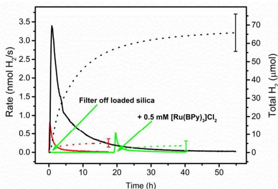
Fig. 2 Hydrogen evolution rate courses (solid lines) and total amounts of H 2 (dotted lines) in 1 M ascorbate buffer (pH 4) with 0.1 M NaOTf. Black: 20 μM 3 and 200 μM 5 adsorbed on hydrophobic fumed silica with 300 μM [C 16 -NMe 3 ][OAc] ( 7 ) as surfactant. Green: Same as black, but loaded silica was filtered off and the residual solution irradiated, then 0.5 mM [Ru(bpy) 3 ]Cl 2 was added and irradiation continued (green arrows). Red: 0.5 mM [Ru(bpy) 3 ]Cl 2 , no WRC. See Table S13.
