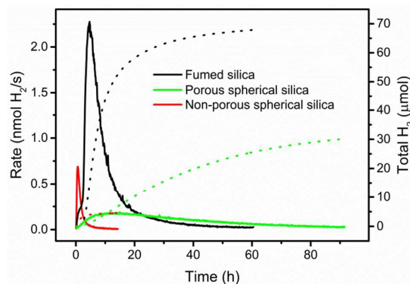
Fig. 6 Comparison of rates (solid lines, left scale) and H 2 amounts (dotted lines, right scale) with WRC 3 and PS 5 immobilized on different types of hydrophobic silica in 1 M ascorbate buffer (pH=4, 0.1 M NaOTf). Black : 200 μM PS 5 and 40 μM WRC 3 on f-SiO 2 -C 18 with 2.5 mM 6 . Red : 4.8 μM 5 and 1 μM 3 on non-porous spherical silica with 100 μM 6 . Green : 200 μM 5 and 40 μM 3 on porous silica with 2.5 mM 6 .
