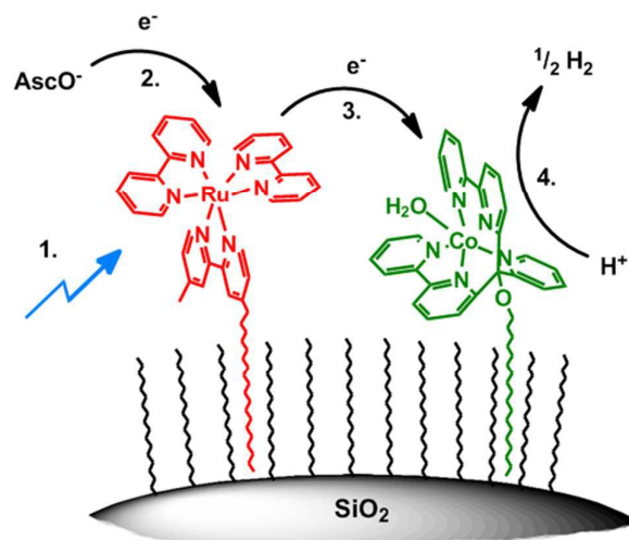
Scheme 4 Proposed reaction mechanism of photocatalytic H 2 production on hydrophobic silica: 1. Photoexcitation of 5 → 5 *; 2. Reductive quenching of 5 * → 5 ; 3. Electron transfer 5 * → 3 ; 4. H + reduction by 3 .
