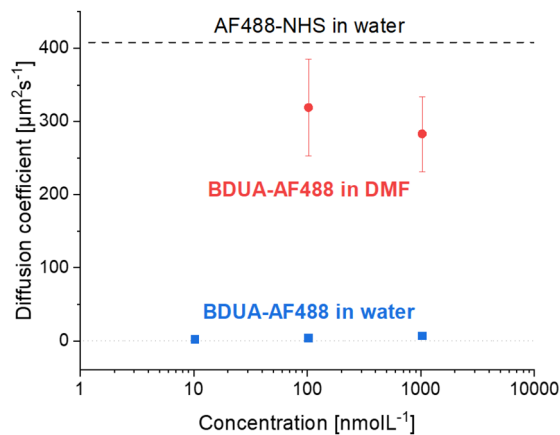
Fig. 7 Comparison of diffusion coefficients derived from autocorrelation data for the reference dye and the supramolecular motif in DMF and water. AF488-NHS was measured at 1.03 nmol L -1 and extrapolated for visualization purposes.
