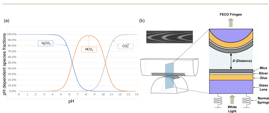
Fig. 1 (a) Fractional concentrations of the three dissolved inorganic carbon (DIC) species present in bicarbonate-containing solutions as a function of electrolyte pH. Calculated using the equilibrium constants as in eqn (1) as shown in the SI. (b) Schematic diagram of the SFB used to measure interactions between mica sheets across electrolyte solution. The mica-coated lens setup is immersed in bulk solution, so that confined system is in equilibrium with a reservoir.
