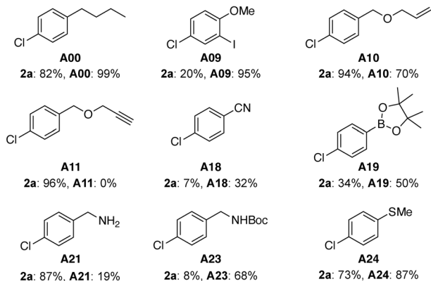
Fig. 3 Additives classified into three groups. The chemical structures of the additives are shown together with the yield of product 2a (%) and recovery rate of additive A (%). (a) Additives leading to decomposition with neither recovery nor product formation ( A04 , A07 , A13 , A14 , A15 , A16 , A20 , and A22 ). (b) Additives showing high recovery but no detectable product 2a ( A01 , A02 , A03 , A05 , A06 , A08 , A12 , and A17 ). (c) Effective additives that afforded product 2a in yields above 5% ( A00 , A09 , A10 , A11 , A18 , A19 , A21 , A23 , and A24 ).
