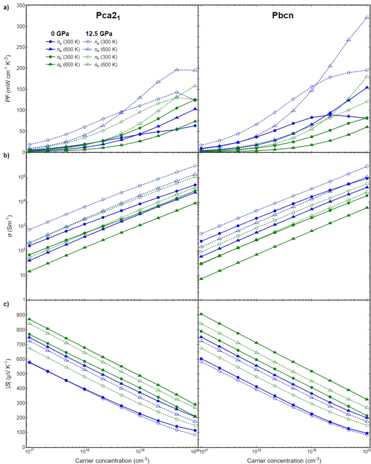
Fig. 5 (a) Power factor (PF), (b) electrical conductivity ( \sigma ), and (c) Seebeck coefficient ( S ) for Pca2_1 (left) and Pbcn BiN polymorph (right). Electronic transport properties are depicted in green and blue for p- and n-type, respectively. Circles and triangles are used for 300 K and 600 K. Properties at 0 GPa and 12.5 GPa are plotted in solid and dashed line, respectively.
