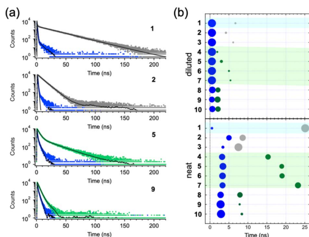
Fig. 5 (a) Time-resolved fluorescence decay curves of liquid samples 1 and 5, and powder samples 2 and 9. Blue traces correspond to diluted samples ( 3 \times 10^{-4} M in chloroform; \lambda_{ex} = 375 nm, \lambda_{em} = 400 nm). Grey and green traces represent neat samples ( \lambda_{ex} = 375 nm, \lambda_{em} = 450 nm for 1; 400 nm for 2 and 3; 500 nm for 4–10). (b) Visual representation of the numerical data presented in Table S3, SI. Blue and green circles indicate the short- and long-lifetime components, respectively, with circle size reflecting their relative contributions.
