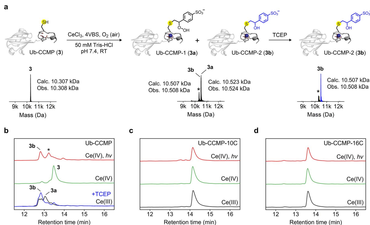
Fig. 5 Cysteine modification with 4VBS on CCMP-tagged ubiquitin. (a) A reaction scheme and LC-MS analysis. The reaction was conducted with 10 \mu\text{M} \text{CeCl}_3 , 10 \mu\text{M} Ub-CCMP (3), and 1 mM 4VBS in 50 mM Tris-HCl, pH 7.4 at 25 ^\circ\text{C} for 12 h, followed by treatment with 1 mM TCEP. HPLC analysis of the reaction products after 12 h using (b) Ub-CCMP, (c) Ub-CCMP-C10, and (d) Ub-CCMP-C16. For photo-irradiated reaction, (\text{NH}_4)_2[\text{Ce}(\text{NO}_3)_6] (CAN) was used instead of \text{CeCl}_3 with 456 nm light. Asterisks shown in a and b indicate Ub-CCMP- \text{SO}_2^- (calc. m/z = 10\ 339 ) or Ub-CCMP- \text{SO}_3^- (calc. m/z = 10\ 355 ).
