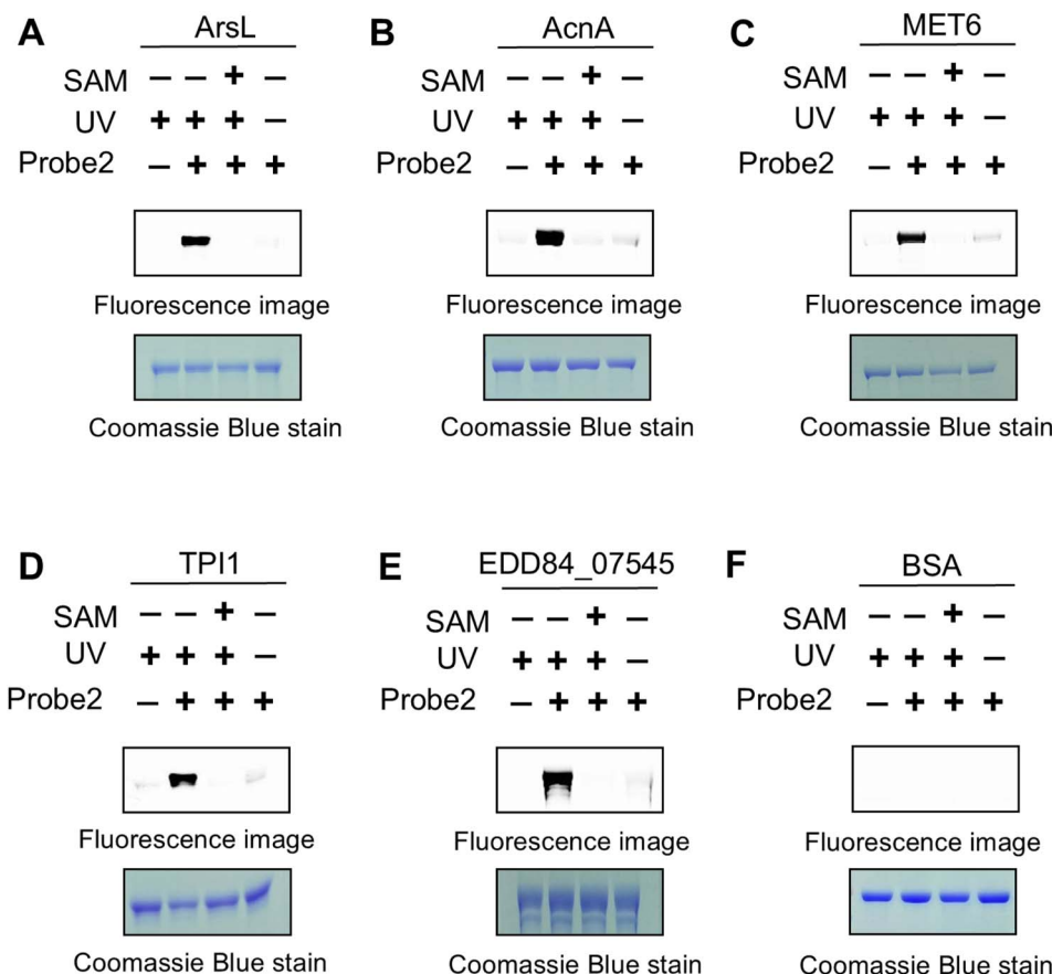
Fig. 6 Verification of five SAM-binding proteins (A–E) and BSA (F) by fluorescence in-gel analysis. Proteins (10 \mu M) were incubated with 100 \mu M probe 2 under UV light irradiation (at 365 nm) before click chemistry. SAM was used as the competitor.
