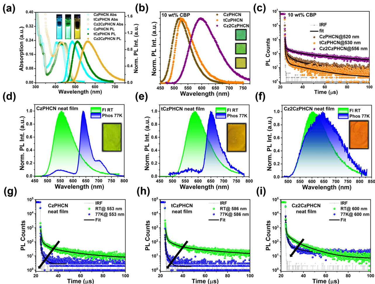
Fig. 3 (a) Absorption and emission spectra of emitters in 10 μM toluene solution. (b) Emission spectra of 10 wt% CBP doped emitters. (c) Delayed lifetime of 10 wt% CBP doped emitters. Fluorescence spectra (green) and phosphorescence spectra (blue) of (d) CzPHCN, (e) tCzPHCN and (f) Cz2CzPHCN in neat film. Delayed lifetime of (g) CzPHCN, (h) tCzPHCN and (i) Cz2CzPHCN at RT (green) and 77 K (blue). All the lifetimes are collected on fluorescence peak maxima. For PL spectra of CzPHCN and tCzPHCN, excitation was 400 nm and for Cz2CzPHCN, 430 nm excitation was used. 355 nm spectralLED was used as the excitation source to measure delayed lifetime.
