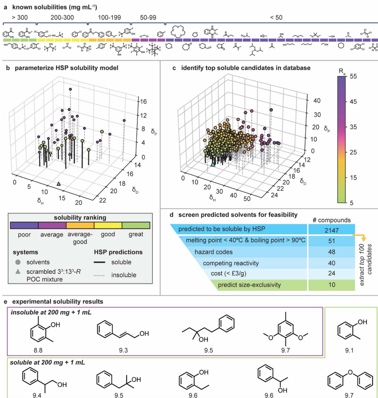
Fig. 3 (a) Curated dataset of existing experimental solubility measurements of 3^3:13^3\text{-R} POC mixture in a range of solvents, including size-excluded examples; (b) the HSP model used to identify the solubility sphere of scrambled 3^3:13^3\text{-R} POC mixture (depicted as the blue triangle). Datapoints are colored based on their solubility ranking. Compounds predicted to form a solubilized mixture are highlighted by a bold, black line; (c) HSP comparison between the POC mixture (triangle data point) and the HSPiP database of candidate solvents (circle datapoints). Candidate solvent molecules are colored by their distance to the scrambled 3^3:13^3\text{-R} POC mixture ( R_a ); (d) solvent down-selection procedure and associated number of candidate compounds remaining at each stage, with the top 10 from this down-selection procedure being selected and taken forward for experimental testing and size-exclusivity prediction; (e) top 10 selected solvents predicted to form a highly soluble mixture with the 3^3:13^3\text{-R} POC which meets all the selection criteria. These predictions were validated experimentally – four candidates were identified to be insoluble at the selected minimum 200 mg + 1 mL threshold (purple) and six candidates were identified to be soluble at 200 mg + 1 mL (green). Each candidate is labelled with its Hansen interaction radius.
