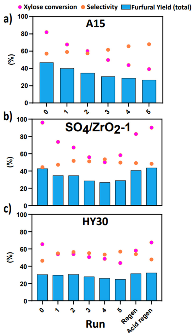
Fig. 2 Cyclic deactivation test for the dehydration of 10 wt% xylose in a H 2 O/MIBK system (1 : 2 by volume) at 160 °C for 2 h at 800 rpm over (a) A15, (b) SO 4 /ZrO 2 -1 and (c) HY30 (2 wt% loading).
