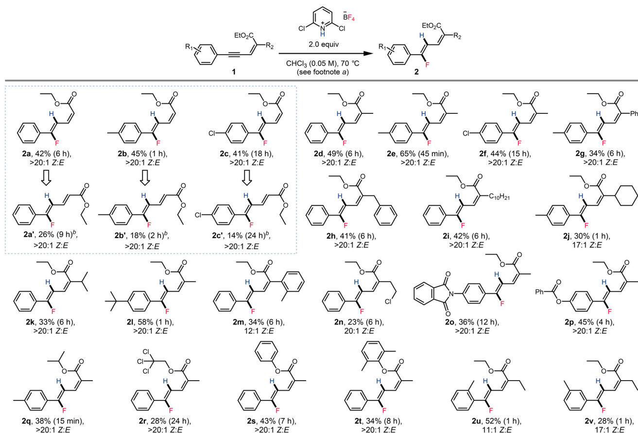
Scheme 2 Substrate scope for the formation of fluorinated dienoates 2 . a Reaction conditions: 1 (0.25 mmol), 2,6-dichloropyridinium tetrafluoroborate (0.50 mmol), chloroform (5.0 mL), stirred at 70 °C for indicated duration. b 1,2-DCE (0.05 M) was used as solvent.
