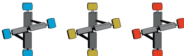
c) decorated cross-shaped tetrachromophores
