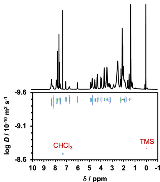
Fig. 3 DOSY NMR spectrum of [2]rotaxane 7. Compound 7 had a single diffusion coefficient, indicating the formation of a rotaxane.
