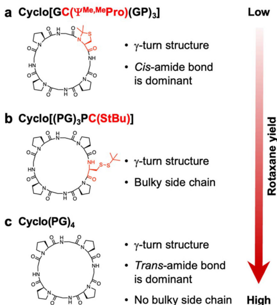
Fig. 5 Summary diagram of the effects of the cyclic peptide amino acid sequence on rotaxane formation in this study. (a) Cyclo[GC( \Psi^{\text{Me,Me}} Pro)(GP) 3 ], which adopts a \gamma -turn structure with predominantly cis -amide bonds (Table 2), was unable to form a rotaxane. (b) Cyclo[(PG) 3 PC(StBu)], which adopts \gamma -turn structure with bulky side chains, formed a rotaxane in a low yield. (c) Cyclo(PG) 4 , which adopts a \gamma -turn structure with predominantly trans -amide bonds (Table 2) and lacks bulky side chains, demonstrated the highest produced a rotaxane in the highest yield to date. This figure underscores how strategically modifying the amino acid sequence modifications in of a cyclic peptide can significantly enhance rotaxane yield. Moreover, continued optimization of these cyclic peptides has the potential to achieve even greater improvements in could lead to further improvements in rotaxane yield.
