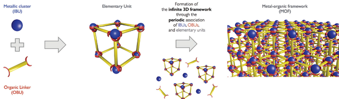
Fig. 3 Conceptual assembly of MOF (reproduced with permission from ref. 32. Copyright 2017, Wiley and Sons).
