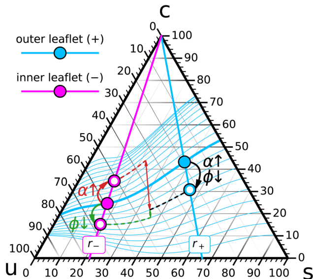
Fig. 5 Perturbation of a ternaary asymmetric GUV initially set up such that its inner composition \{r_-, \phi_-\} (big magenta dot) and outer composition \{r_+, \phi_+\} (big cyan dot) chemically coexist at \mathcal{F} = 0 . The two independent perturbations which either decrease \phi or increase \alpha will have a similar effect on leaf _+ : a reduction of \phi_+ . But their effects on leaf _- are opposite: depleting cholesterol will reduce \phi_- while increasing \alpha will increase \phi_- . The extent to which this moves points that originally shared the same zero-torque foliation onto different foliation curves is very different.
