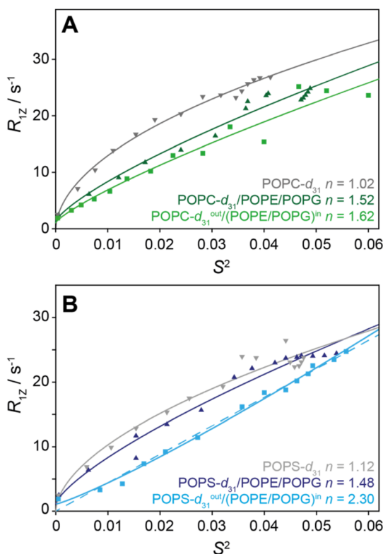
Fig. 3 (A) Square law plots of POPC- d_{31}^{\text{out}}/(\text{POPE}/\text{POPG})^{\text{in}} membranes (light green squares), symmetric POPC- d_{31}/\text{POPE}/\text{POPG} bilayers (dark green triangles), and pure POPC- d_{31} membranes (gray upside down triangles). (B) Square law plots of POPS- d_{31}^{\text{out}}/(\text{POPE}/\text{POPG})^{\text{in}} membranes (light blue squares), symmetric POPS- d_{31}/\text{POPE}/\text{POPG} bilayers (dark blue triangles), and pure POPS- d_{31} membranes (light gray upside down triangles). The lines represent best fits to the function R_{1Z} = y_0 + a \times S^n , and the dashed solid line represents a linear regression.
