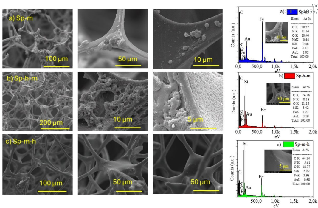
Figure 2. SEM images and the corresponding EDX spectra of the a) Sp-m, b) Sp-h-m and c) Sp-m-h samples.
