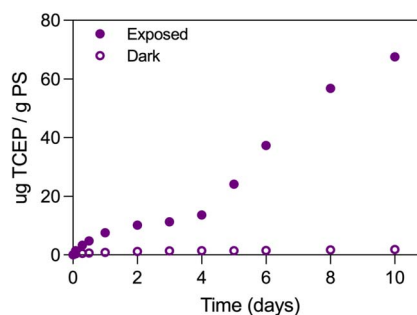
Fig. 3 Concentration of TCEP detected in the leachate of a 1 w/w% TCEP-PS composite suspended in water and exposed to \text{UV}_{300\text{nm}} irradiation (closed circles) or under dark conditions (open circles).
