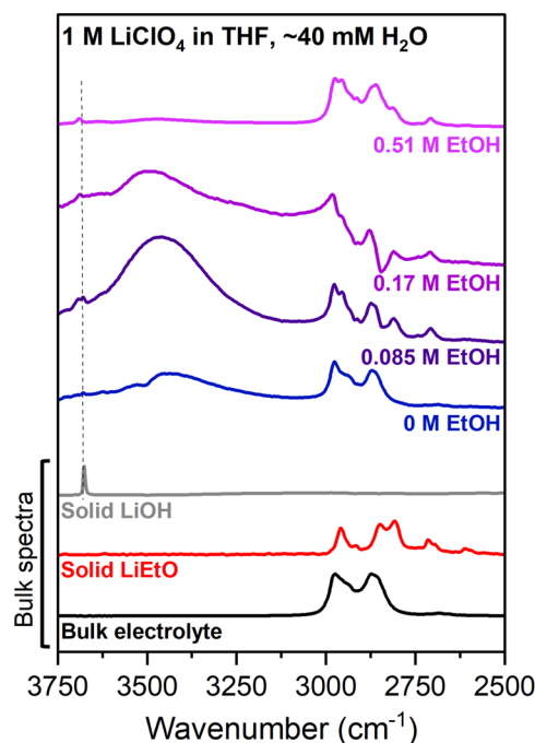
Fig. 4 Comparison of the in situ FTIR spectra of the SEIs taken near Li plating potential in electrolytes of 1\text{ M LiClO}_4 in THF containing approximately 40\text{ mM} water (medium concentration) with ethanol concentrations of 0 , 0.085 , 0.17 and 0.51\text{ M} , corresponding to 0\% , 0.5\% , 1\% and 3\% ethanol by volume respectively. All spectra are relative to spectra measured at the initial open circuit potential in each experiment (approx. +3.3\text{ V} vs. \text{Li/Li}_{\text{app}}^+ ). The bulk spectra of the electrolyte and pure \text{LiOH} and \text{LiEtO} were measured using an ATR accessory inside an Ar glove box.
