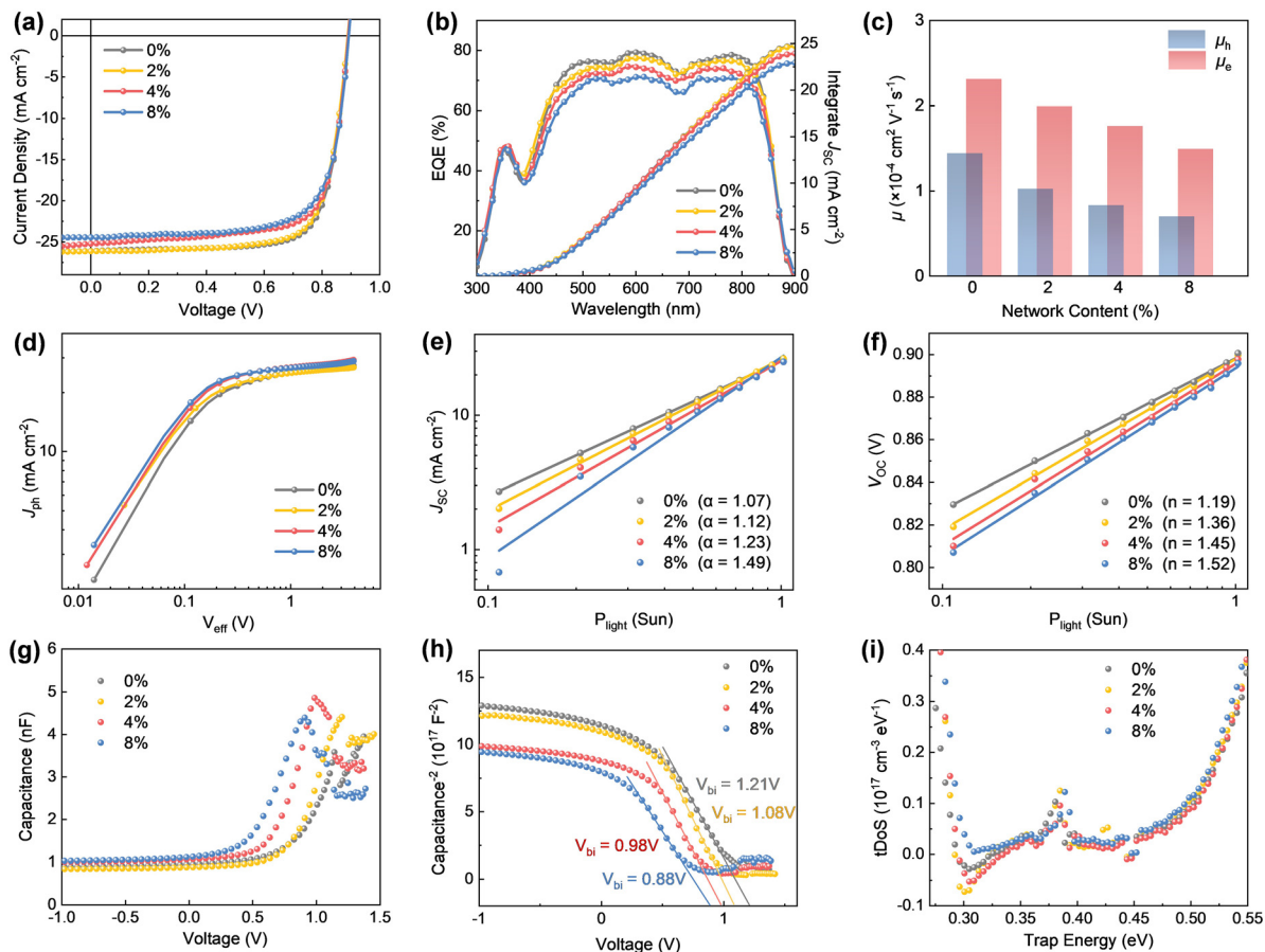
Fig. 3 (a) J - V curves and (b) EQE spectra of OSCs fabricated with varying BVTD ratios. (c) SCLC mobilities of active layer thin films prepared with different BVTD ratios. (d) J_{\text{ph}}-V_{\text{eff}} curves, and P_{\text{light}} dependence of (e) J_{\text{SC}} and (f) V_{\text{OC}} for OSCs, where 1 sun corresponds to P_{\text{light}} = 100 \text{ mW cm}^{-2} . (g) C-V characteristics of OSCs with varying BVTD ratios. (h) 1/C^2-V plots derived from the C-V curves. (i) tDoS as a function of E_{\text{tr}} derived from C-F characteristics.
