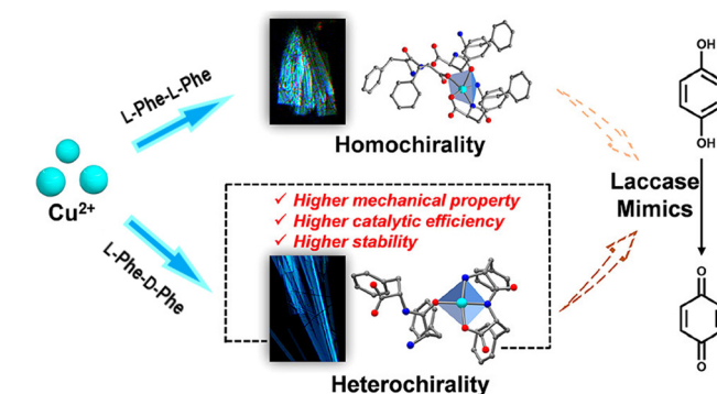
Fig. 29 Schematic illustration of the chirality-dependent coordination assembly process between Phe-Phe molecules and Cu 2+ , in which the peptide heterochirality leads to enhanced properties of a laccase mimic. Reproduced and adapted from ref. 245 with permission from American Chemical Society, copyright 2022.
