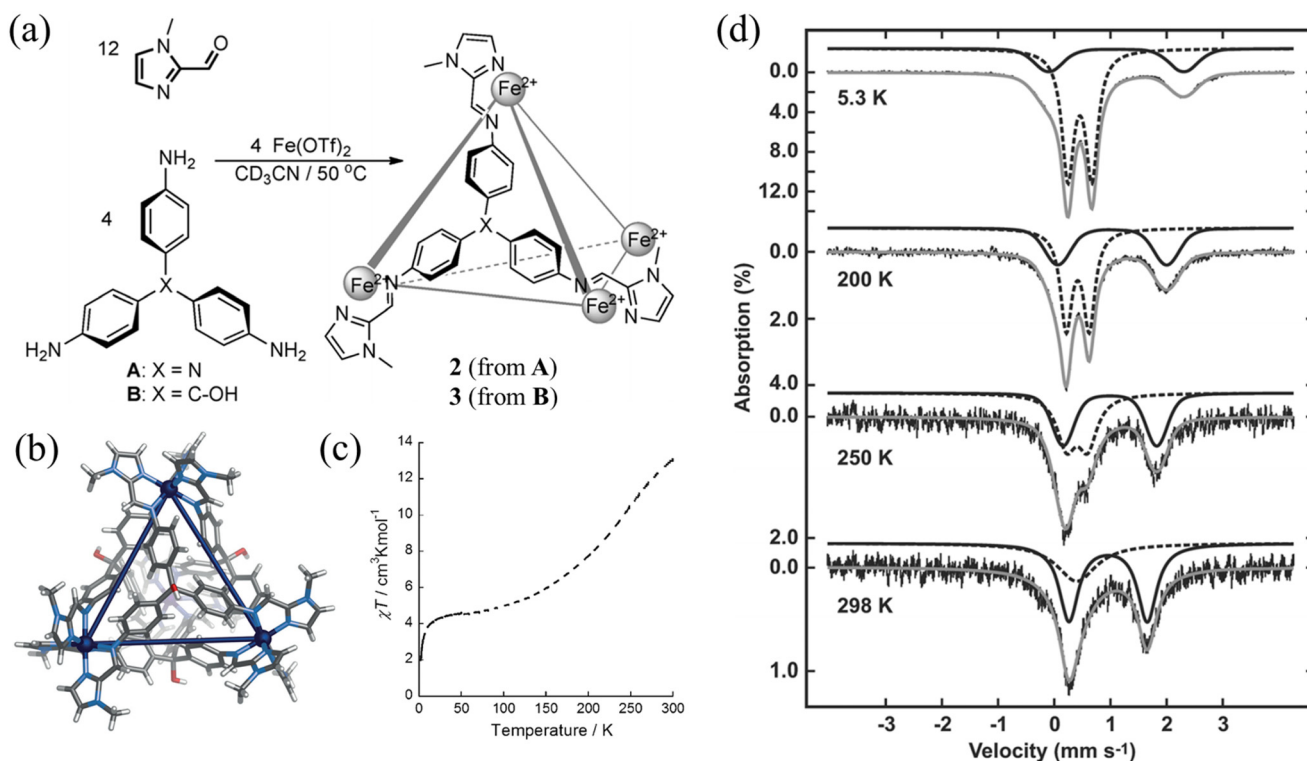
Fig. 5 (a) Synthesis method of cages 2 and 3 . (b) Crystal structure of cage 2 . \chi_m T vs. T plots (c) and variable-temperature ^{57}\text{Fe} Mössbauer spectra (d) for cage 2 . Adapted from ref. 77.
