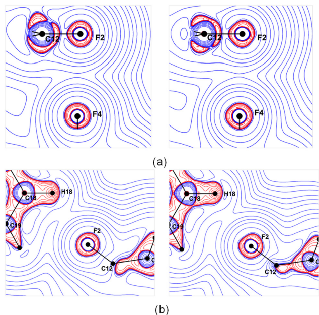
Fig. 7 Experimental (left) and theoretical (right) Laplacian maps for (a) C12-F2...F4-C10 interaction and (b) C18-H18...F2-C12 hydrogen bond drawn at the logarithmic interval of -\nabla^2\rho \text{ e } \text{\AA}^{-5} .
