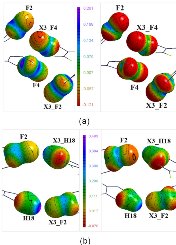
Fig. 8 Experimental (left) and theoretical (right) 3D ESP maps for (a) the C12-F2...F4-C20 interaction and (b) C18-H18...F2-C12 hydrogen bond plotted at an interval of \pm 0.1 \text{ e } \text{\AA}^{-3} .
