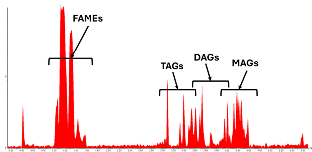
Fig. 10 Base peak ion current chromatogram (BPIC) of the positive ion ESI SFC-MS for HVO 6.
