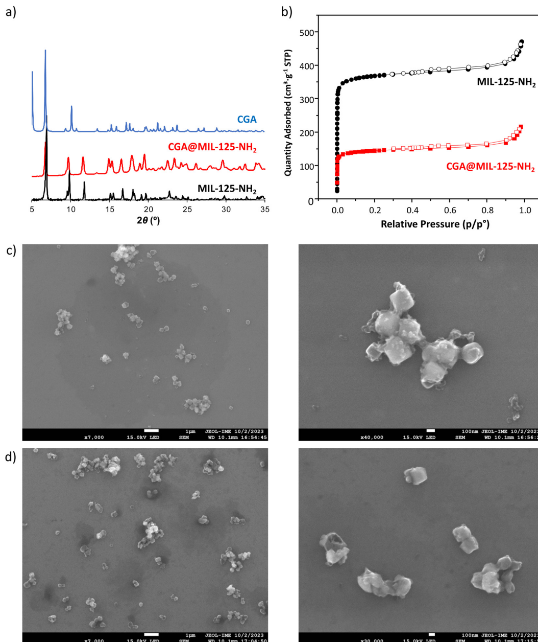
Fig. 1 (a) XRPD patterns of pristine and CGA loaded MIL-125-NH 2 . Free CGA XRPD pattern was added for comparison. (b) N 2 sorption isotherms (77 K) for MIL-125-NH 2 before (black, circles), and after (red, squares) the CGA loading. Empty symbols denote desorption. FE-SEM images of (c) MIL-125-NH 2 and (d) CGA@MIL-125-NH 2 . No significant differences are observed in the cubic shaped particles.
