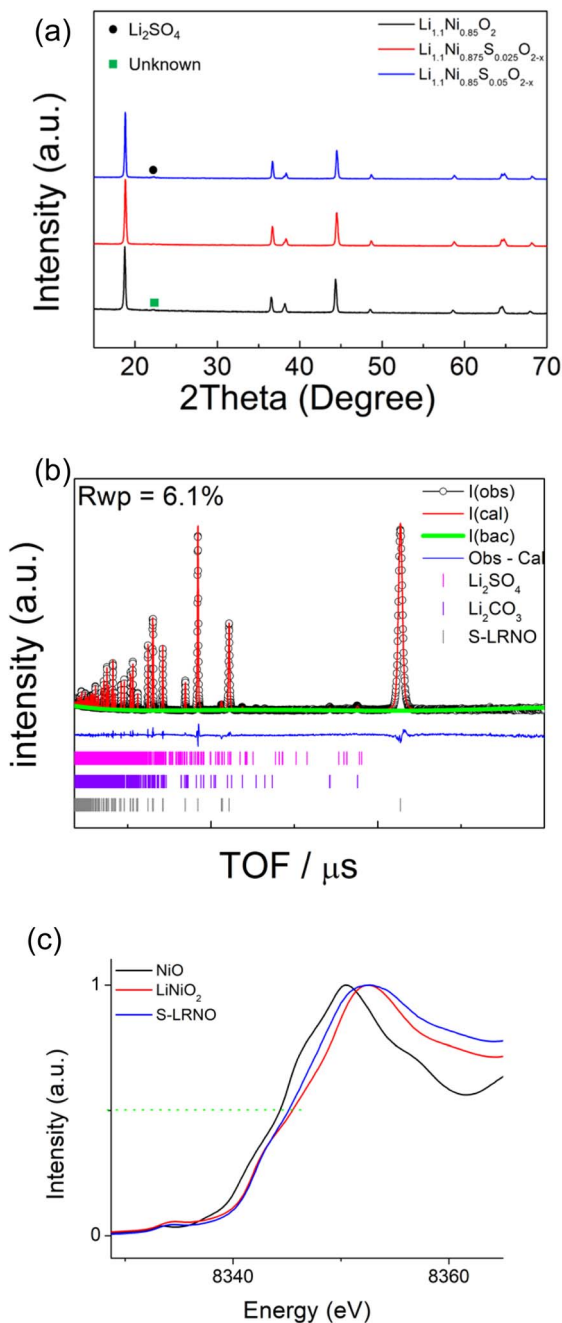
Fig. 2 (a) XRD patterns of Li 1.1 Ni 0.85 O 2 , Li 1.1 Ni 0.875 S 0.025 O 2-x and Li 1.1 Ni 0.85 S 0.05 O 2-x (solid state synthesis route). (b) Observed, calculated and difference profiles from structural refinement of Li 1.1 Ni 0.85 S 0.05 O 2-x using neutron diffraction data (c) XAS data of Li 1.1 Ni 0.85 S 0.05 O 2-x .
