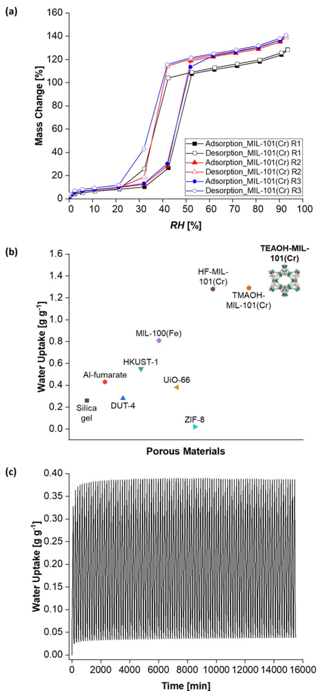
Fig. 7 (a) Water adsorption–desorption isotherms ( T = 25\text{ °C} ) of TEOH-MIL-101(Cr) where the water uptake capacity increases with additional rounds of washing in warm ethanol. (b) Water uptake of various MOFs at T = 25\text{ °C} and RH = 90%. The water uptake of silica gel under the same conditions is included for comparison. (c) Cyclic performance of TEOH-MIL-101(Cr) R3 over 100 adsorption–desorption cycles with 90 min of adsorption at T = 25\text{ °C} and RH = 50% followed by 65 min of desorption at T = 50\text{ °C} and RH = 0%.
