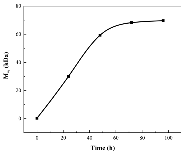
Fig. 4 Change of PRA molecular weights during polymerization (conditions: MR : [OdmMIM][NTf 2 ] = 1 : 1 in mole, 1 wt% of TIP as the catalyst, 180 °C).
