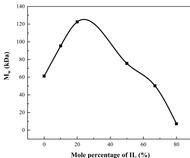
Fig. 5 Polycondensation of MR in different amounts of [OdmMIM][NTf 2 ] (conditions: TBT as the catalyst, 180 °C, 72 h).
