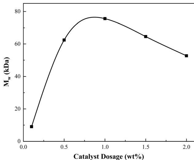
Fig. 3 Solution polycondensation of MR in [OdmMIM][NTf 2 ] with different catalyst dosages (conditions: TBT used as the catalyst, MR : [OdmMIM][NTf 2 ] = 1 : 1 in mole, 180 °C, 72 h).
