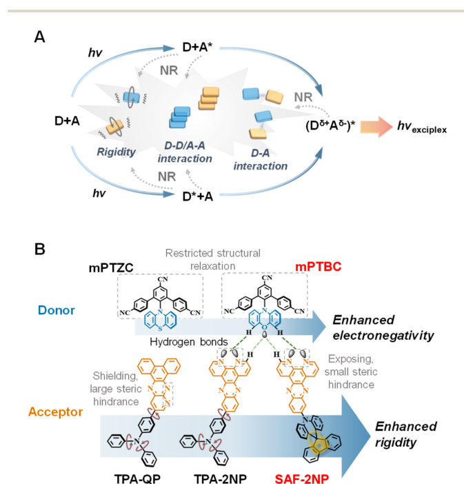
Fig. 1 (A) Illustration of the emission process of exciplex emitters and three factors that can lead to non-radiative decay of exciplex emitters. D stands for donors, A represents acceptors and NR is non-radiative decay. (B) Design concept and the corresponding molecular structures of donors and acceptors.
