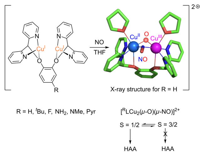
Fig. 10 Synthesis of [\text{R}^{\text{I}}\text{LCu}_2(\mu\text{-O})(\mu\text{-NO})]^{2+} species and influence of the spin state on HAA reactivity from ref. 73 and 74.
