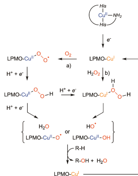
Scheme 3 Putative mechanisms to explain LPMO catalyzed hydroxylation: (a) the monoxygenase pathway and (b) peroxigenase pathway.
