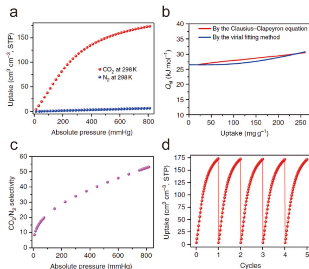
Fig. 34 (a) The CO 2 and N 2 adsorption isotherms for FJI-H14 at 298 K. (b) The isosteric heat of CO 2 adsorption (Q st ) for FJI-H14. (c) The IAST selectivity of FJI-H14 for CO 2 /N 2 (15:85). (d) 5 Cycles of CO 2 adsorption for FJI-H14 at 298 K. Reproduced from ref. 136 with permission from Springer Nature, Copyright 2017.
