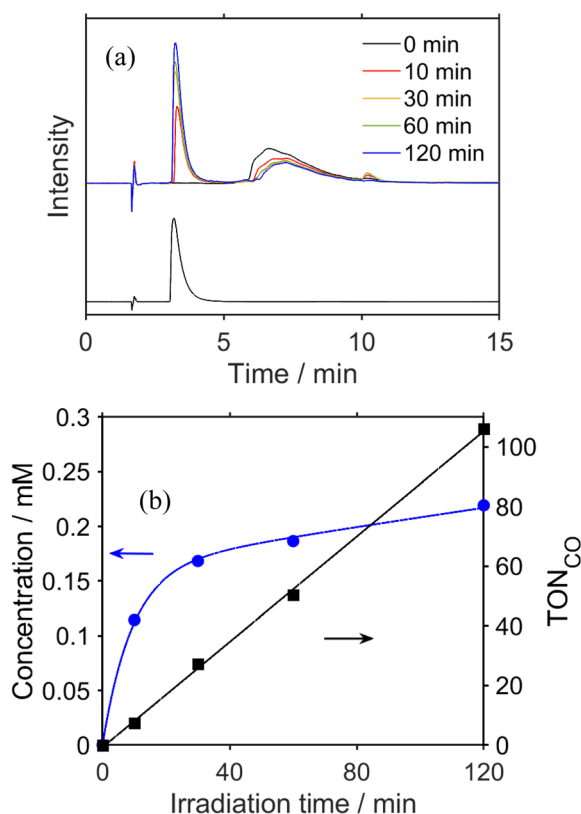
Fig. 5 (a) UHPLC chromatograms of (top) a \text{CO}_2 saturated DMSO-TEOA (5 : 1 v/v) solution containing RuC2Re (0.5 mM) and BIH (0.1 M) before and after irradiation at 490–620 nm ( \lambda_{\text{max}} = 530 nm) for various irradiation times; the chromatogram of a DMSO-TEOA (5 : 1 v/v) solution containing RuC2Re(CO) is shown at the bottom (ODS; eluent: \text{MeOH-KH}_2\text{PO}_4 buffer (pH = 5.9); detection wavelength \lambda_{\text{det}} = 460 nm). (b) Concentration change of the accumulated RuC2Re(CO-TEOA) , which was observed as RuC2Re(CO) in the UHPLC analysis (blue) and TON of CO formation (black) during irradiation.
