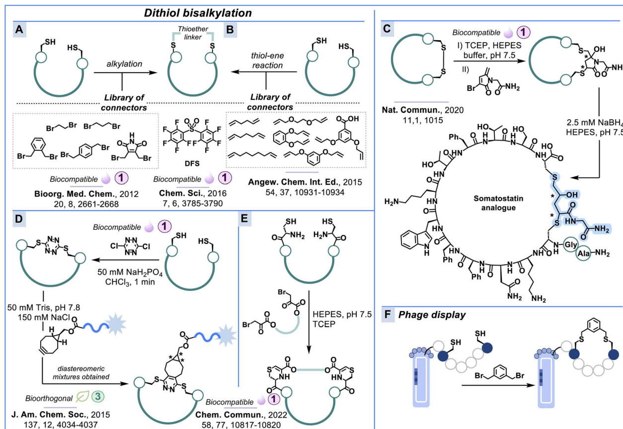
Scheme 4 Peptide dithiol bisalkylation. Bridging two cysteine residues using [A] haloalkyl connectors or [B] di-ene to perform thiol-ene chemistry. [C] Cysteine stapling with a 3-bromo-5-methylene pyrrolone derivative. [D] S,S -Tetrazine staples allow further modification under bioorthogonal conditions. [F] Cysteine stapling during phage display with DBMB.
