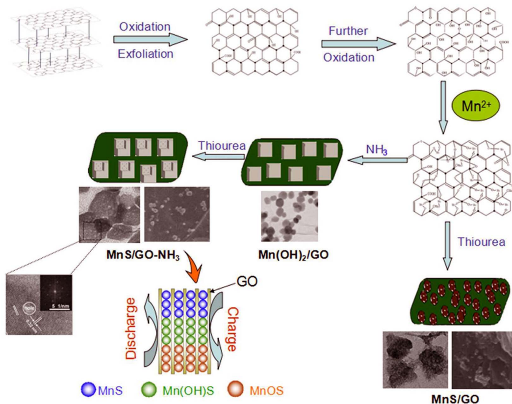
Fig. 5 Schematic of the preparation processes of \text{MnS/GO-NH}_3 and \text{MnS/GO} composites. 156
