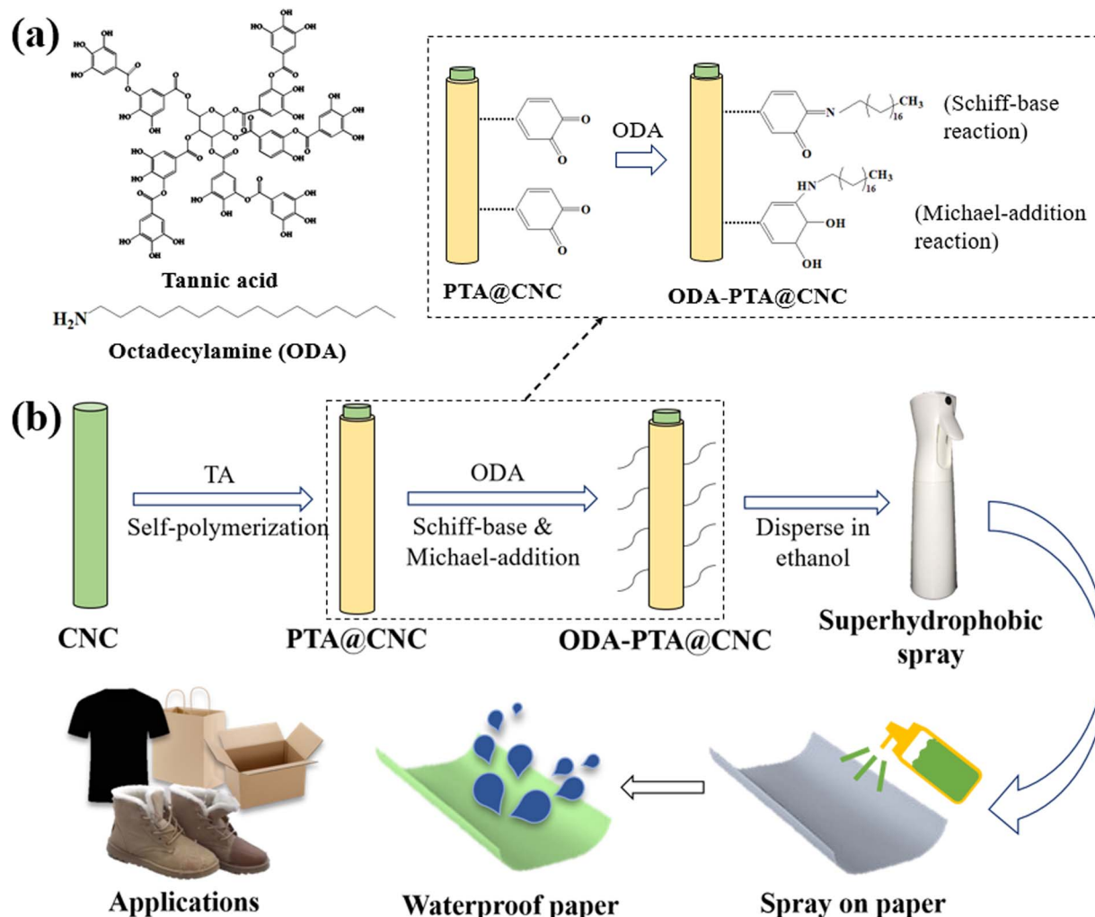
Fig. 17 (a) Chemical reaction occurring the of preparing superhydrophobic coating. (b) Schematic representation of preparing superhydrophobic coating using CNCs (PTA@CNCs) and ODA and its applications. 112 Reproduced from ref. 112 with permission from ACS Sustainable Chemistry & Engineering, copyright 2022.
