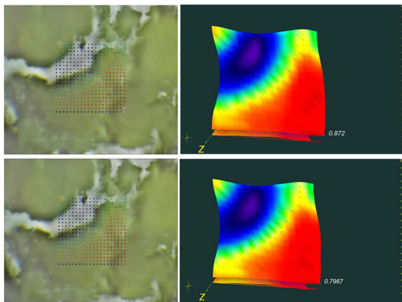
Fig. 4 ATR-FTIR mapping for [Rut \subset \beta -CD] complex powder. Mapping area is 302 × 302 microns. 15× ATR objective.
