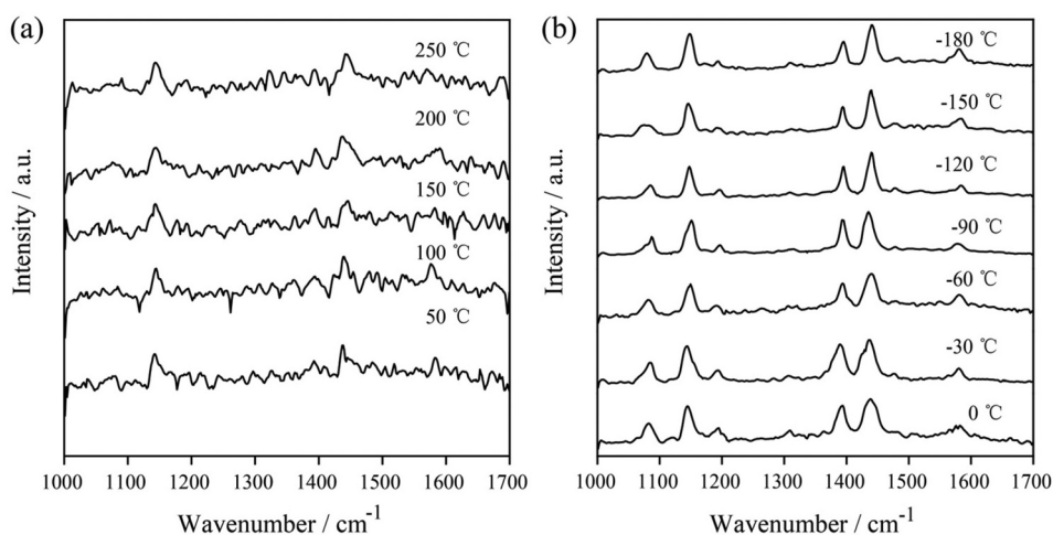
Fig. 6 Temperature-dependent SERS spectra of the plasmon-induced photocatalytic reaction of 4-ATP at 50–250 °C (a) and at –180–0 °C (b) with 532 nm excitation ( P = 1.05\ \mu\text{W} , t_{\text{acq}} = 60 s).
