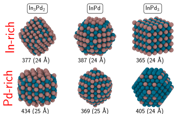
Fig. 3 Morphologies of \text{In}_3\text{Pd}_2 (left), \text{InPd} (middle) and \text{InPd}_3 (right) NPs based on the Wulff construction. The diameter of each NP is given, along with its number of atoms. The top row corresponds to the NP morphology at the In-rich side whereas the bottom row corresponds to the Pd-rich side. Colour code: Pd = blue and In = brown.
