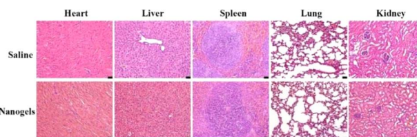
Fig. 7 Histological images of the major organs of Balb/c mice after treatment for 2 weeks. The scale bars at the right corner are 20 \mu m.
