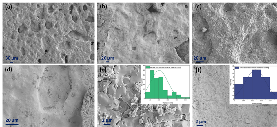
Fig. 10 Surface SEM images of (a), (c) and (e) 100-layer and (b), (d) and (f) drop-cast porous NLK–GDC symmetric cells in 185 \times (a and b), 687 \times (c and d), and 4.15k \times (e and f) magnifications. The insets of (e) and (f) figures are the particle size distributions of CuFe 2 O 4 particles on the surface of the inkjet-printed and drop-cast samples, respectively, analyzed using ImageJ software.
