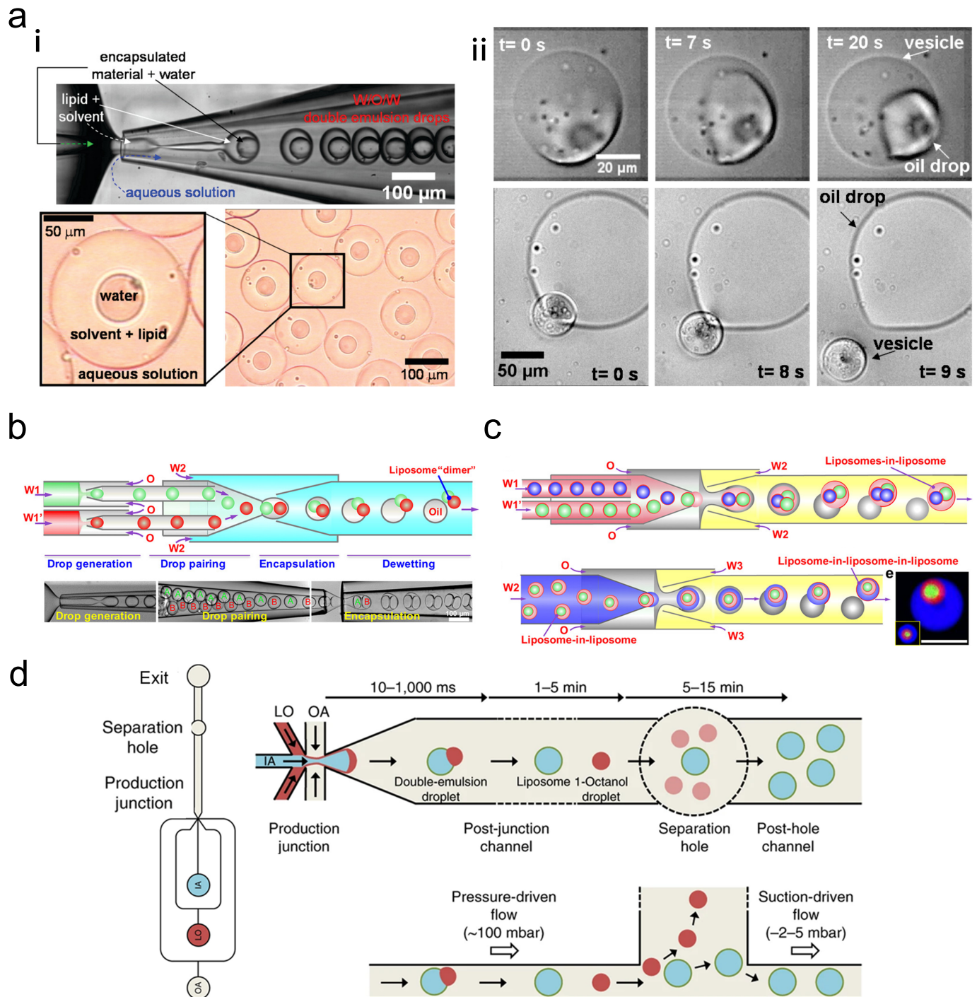
Fig. 11 Microfluidic double emulsion-based vesicle generation. a) (i) Top: Formation of phospholipid-stabilized W/O/W double emulsion in a glass microcapillary device. Bottom: Optical micrograph of the double emulsion collected. (ii) Top: Vesicle formation through solvent drying on the vesicle surface. Excess phospholipid is concentrated in the remaining oil drop attached to the resulting vesicle. Bottom: Release of a vesicle from a double emulsion drop pinned on a glass slide. The oil drop that contains excess phospholipids remains on the glass slide. Reproduced from Ref162 with permission from the American Chemical Society, copyright[2008]. b) Fabrication of liposomes with distinct multicompartment structures. Schematic (top) and snapshots (bottom) of the fabrication of double emulsions with two distinct droplets. Scale bars are 100 \mu\text{m} . Reproduced from Ref166 with permission from the American Chemical Society, copyright[2016]. c) Top: Schematics of the microfluidic preparation of double emulsions with distinct interior liposomes (liposomes-in-liposome) and the dewetting process. Bottom: The formation of triple vesosomes (liposome-in-liposome-in-liposome) and the resultant structures. Scale bars, 100 \mu\text{m} . Reproduced from Ref167 with permission from the American Chemical Society, copyright[2017]. d) Schematics showing octanol-assisted liposome assembly (OLA) vesicle production and purification. An overall layout of the microfluidic device and the post-junction channel (left). A top view (right top) and a side view (right bottom) of the OLA junction. IA, inner aqueous phase; LO, lipid-carrying organic phase; OA, outer aqueous phase. Reproduced from Ref172 with permission from Springer Nature, copyright[2016].
