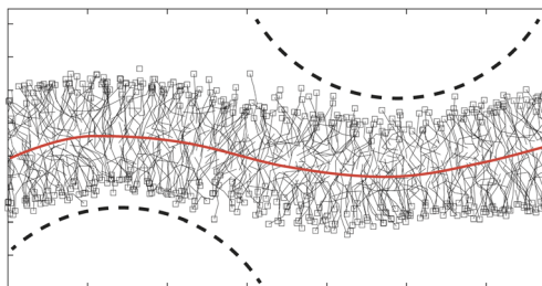
Fig. 2 Simulation snapshot of a symmetric and tensionless bilayer. The lipid bilayer has a thickness of about 4 nm. The smallest curvature radius of its mid-surface (red) is about 6 nm, the radius of the dashed circles. Reused with permission from ref. 14, American Physical Society, 1999.
