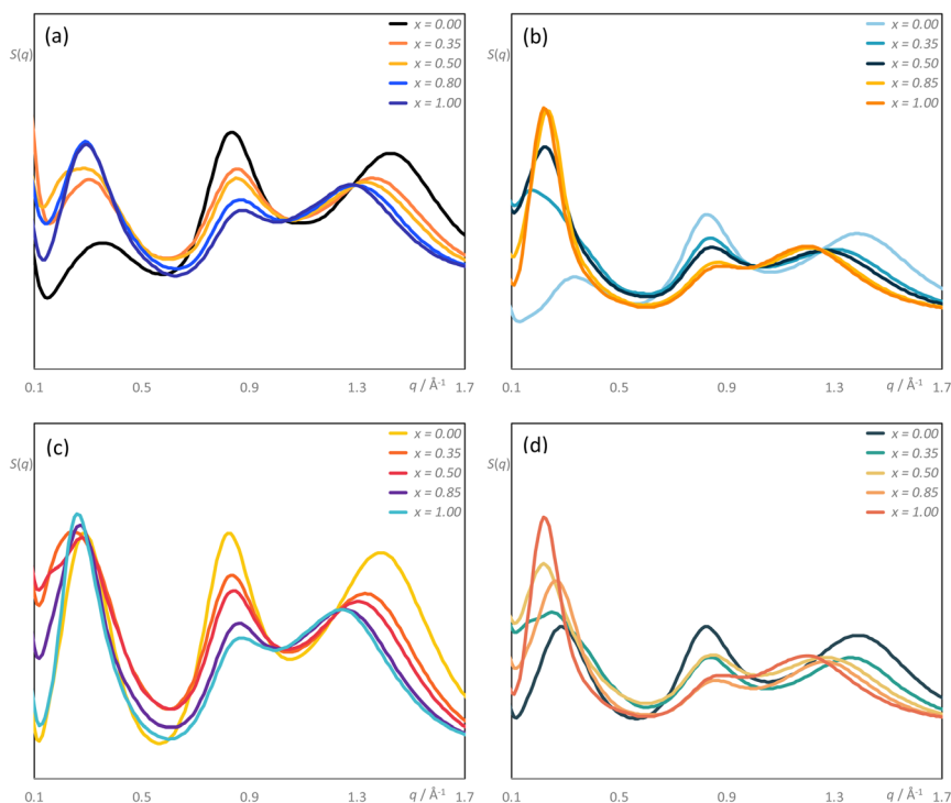
Fig. 9 Total structure factor functions, S(q) : (a) [\text{C}_8\text{MIM}]_{1-x}[\text{C}_{10}\text{MIM-F}_{17}]_x[\text{TF}_2\text{N}] ; (b) [\text{C}_8\text{MIM}]_{1-x}[\text{C}_{10}\text{MIM-F}_{13}]_x[\text{TF}_2\text{N}] ; (c) [\text{C}_{10}\text{MIM}]_{1-x}[\text{C}_8\text{MIM-F}_{13}]_x[\text{TF}_2\text{N}] ; (d) [\text{C}_{10}\text{MIM}]_{1-x}[\text{C}_{10}\text{MIM-F}_{17}]_x[\text{TF}_2\text{N}] mixtures. Data for (a) at 300 K and for (b) to (c) at 333 K.
