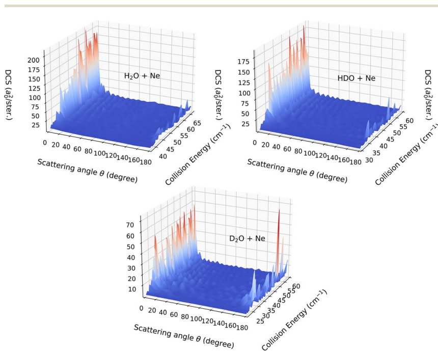
Fig. 9 Differential cross section for the ( 1_{11} \leftarrow 0_{00} ) transitions induced by the collision of H 2 O, HOD or D 2 O with Ne.
