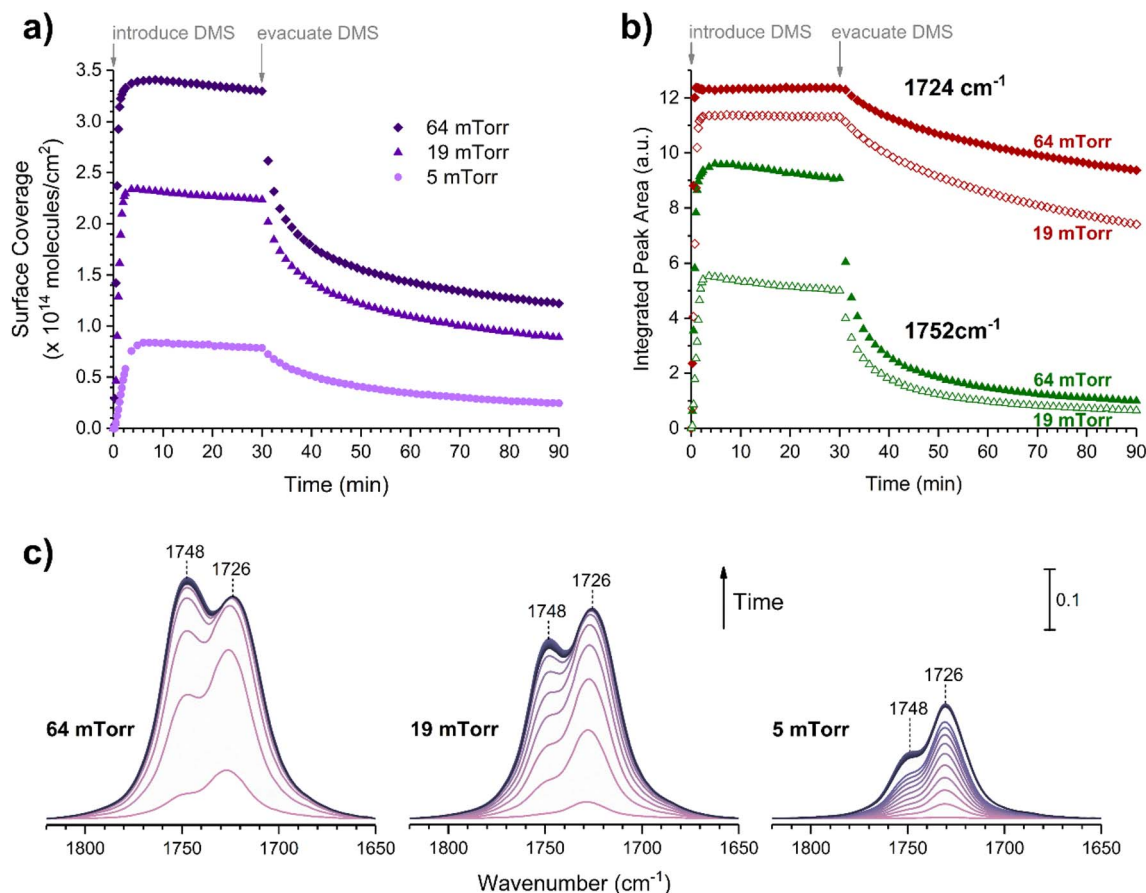
Fig. 4 (a) Temporal surface coverages of adsorbed DMS on the \text{SiO}_2 surface at equilibrium pressures of 5, 19, and 64 mTorr. The surface was exposed to DMS for 30 min, then evacuated for 1 h. (b) Temporal integrated surface areas of deconvoluted C=O bands centered at 1724 \text{cm}^{-1} (red) and 1752 \text{cm}^{-1} (green) from the FTIR spectra of \text{SiO}_2 surfaces exposed to DMS at 19 mTorr (open markers) and 64 mTorr (solid markers). (c) Temporal FTIR spectra of \text{SiO}_2 surfaces exposed to DMS at 5, 19, and 64 mTorr.
