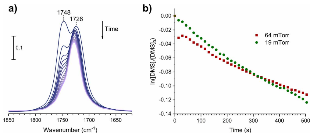
Fig. 5 (a) Temporal desorption FTIR spectra during a 1 h evacuation after the \text{SiO}_2 surface was exposed to DMS at 64 mTorr for 30 min. (b) First-order desorption kinetics of DMS from \text{SiO}_2 surfaces following their exposures at 19 and 64 mTorr.
