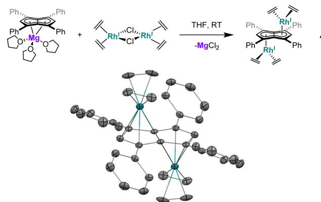
Fig. 3 Synthesis of anti -[Rh'(C 2 H 4 ) 2 ][μ:η 5 :η 5 Ph 4 Pn] (4) (top) and its X-ray crystal structure with thermal ellipsoids at the 50% probability level (bottom; hydrogen atoms omitted for clarity).
