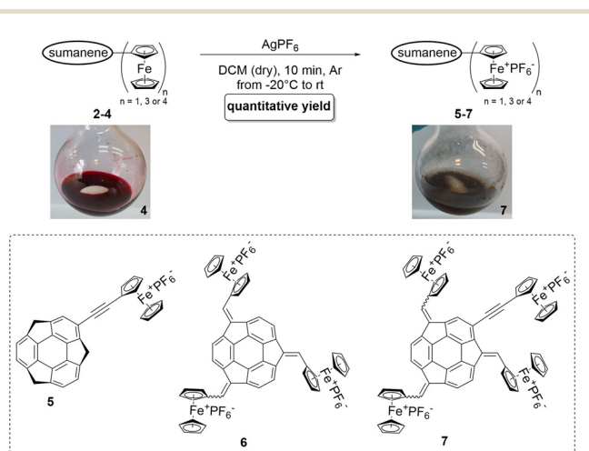
Fig. 4 Oxidation of the sumanene-ferrocene conjugates 2–4 to \text{Fc}^+ -containing compounds 5–7 . Solution colours before and after the reaction in the representative synthesis of 7 from 4 are also presented.
